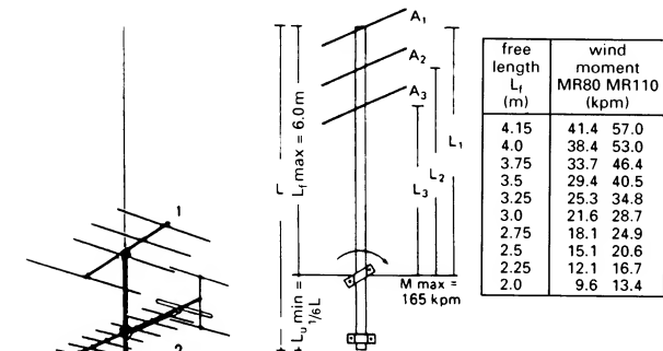
④ Wind moment MR on a vertical tube with 50 mm diameter
